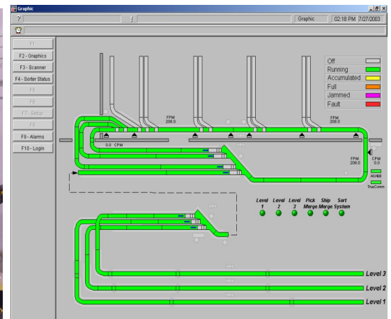
TrueSort® Graphical HMI Screen
