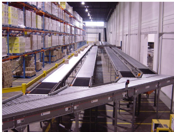
Shipping Merge Area
